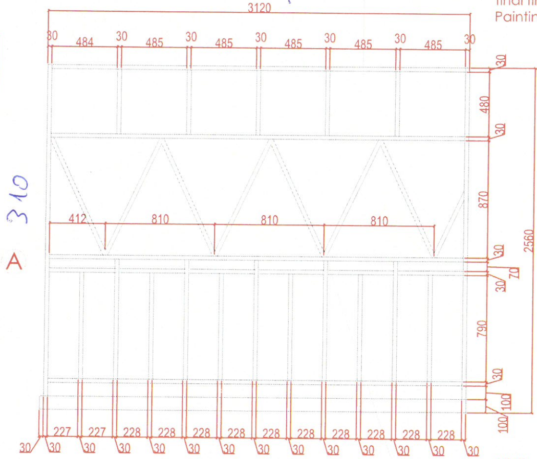
FRONT Elevation-A Details
